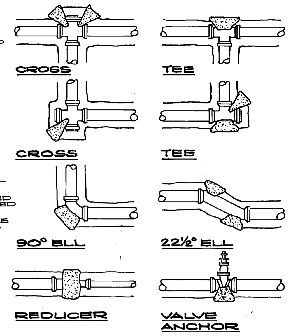
THRUST BLOCK DETAILS NO SCALE
