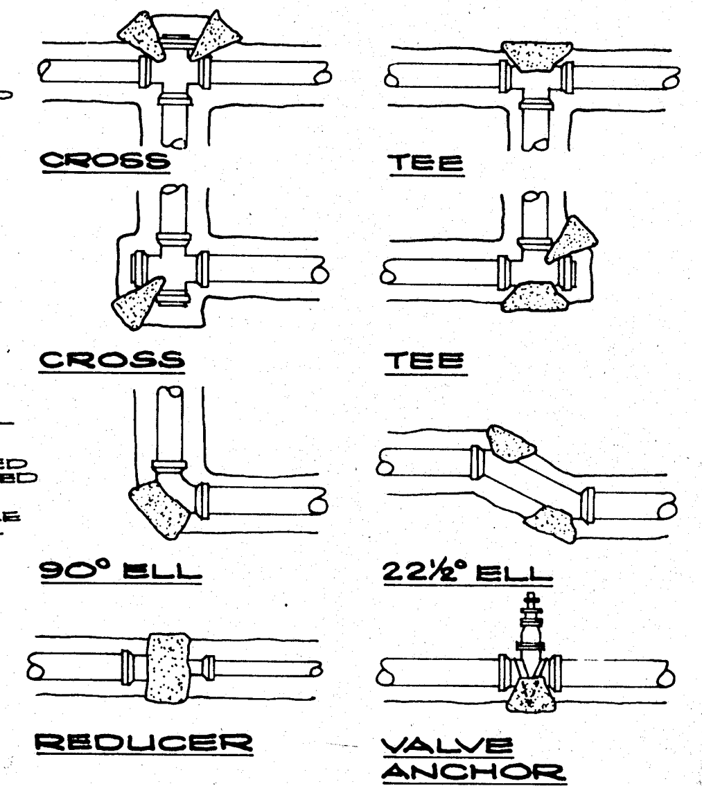
THRUST BLOCK DETAILS
