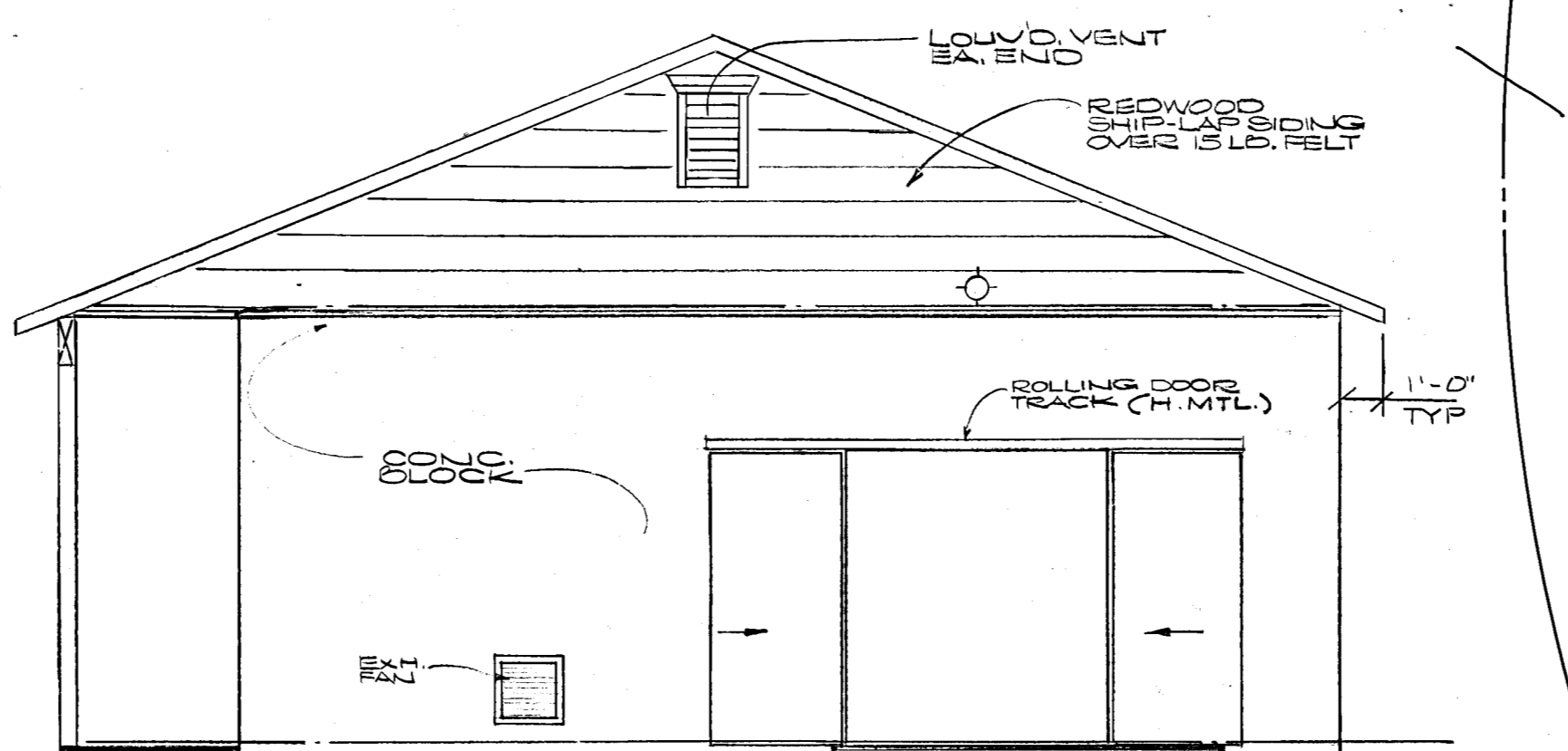
SOUTH ELEVATION
