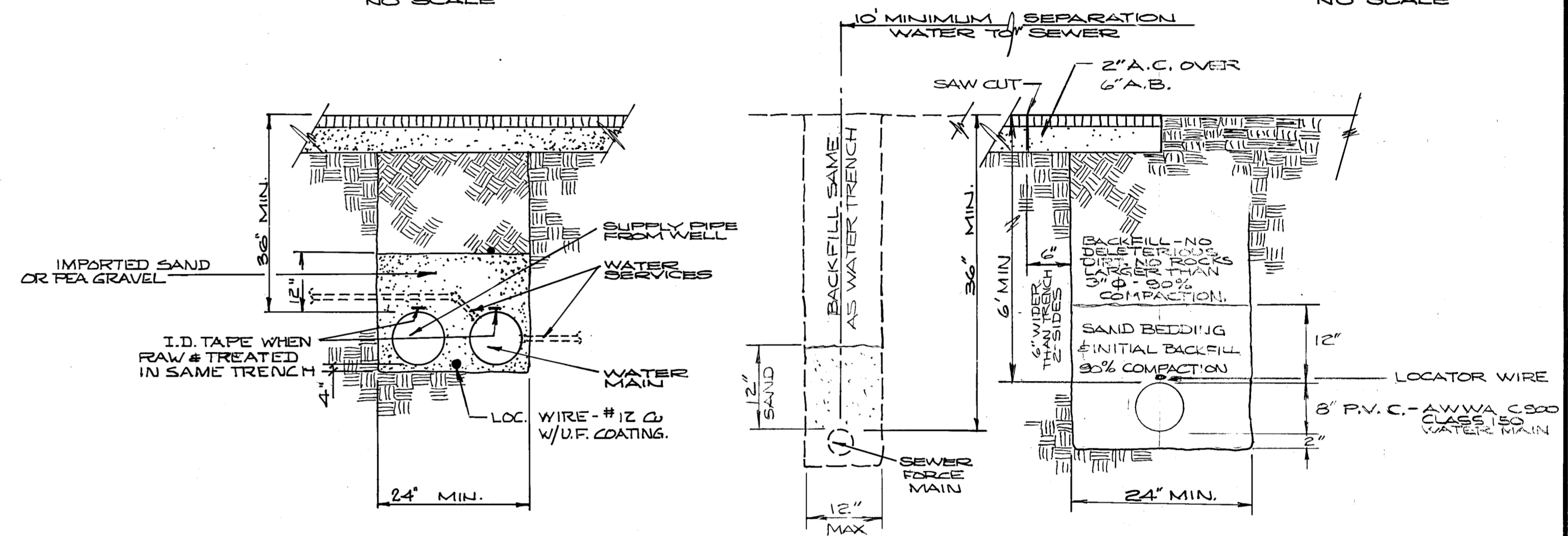
WATER TRENCH DETAIL NO SCALE
