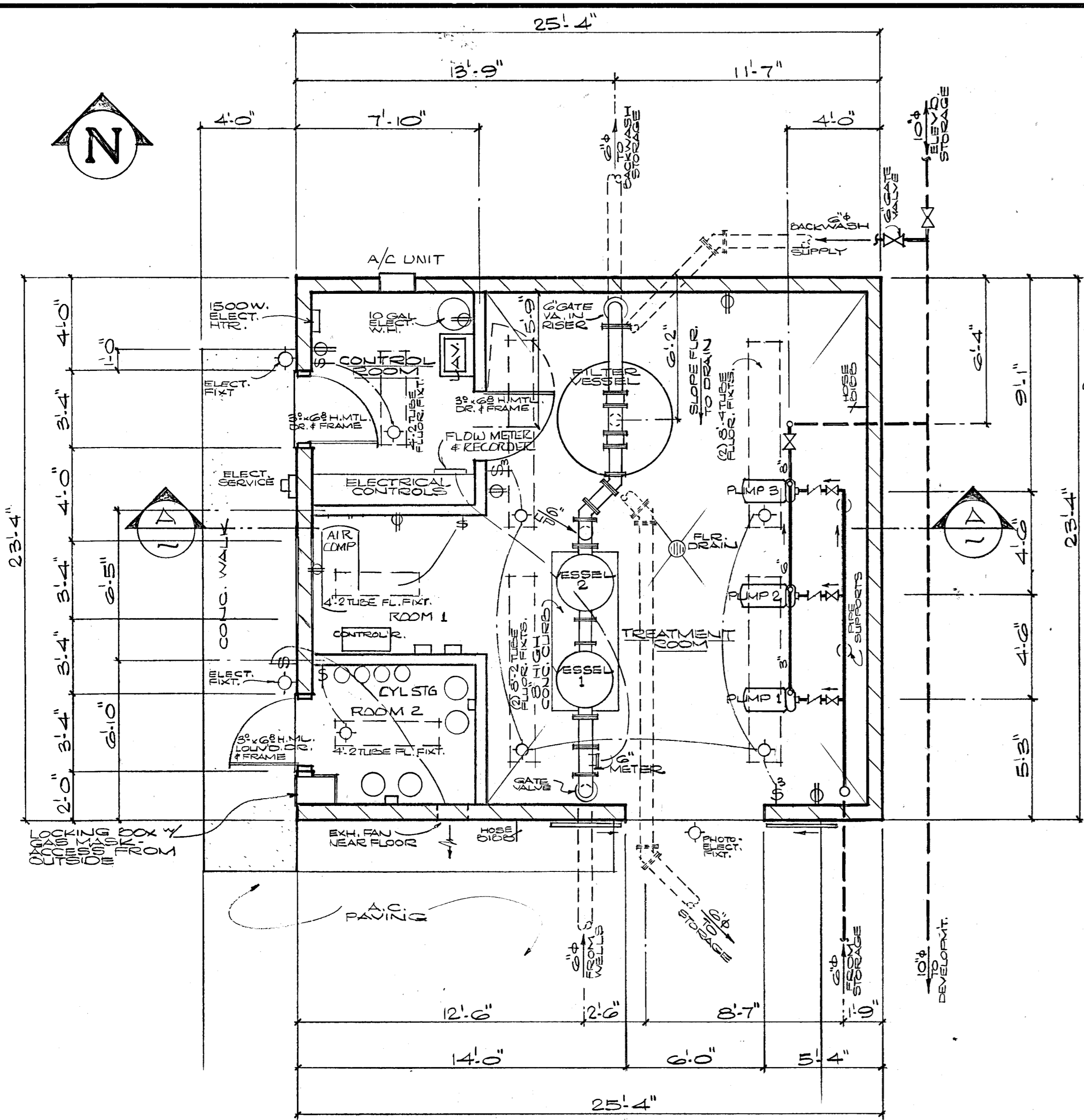
FLOOR PLAN
