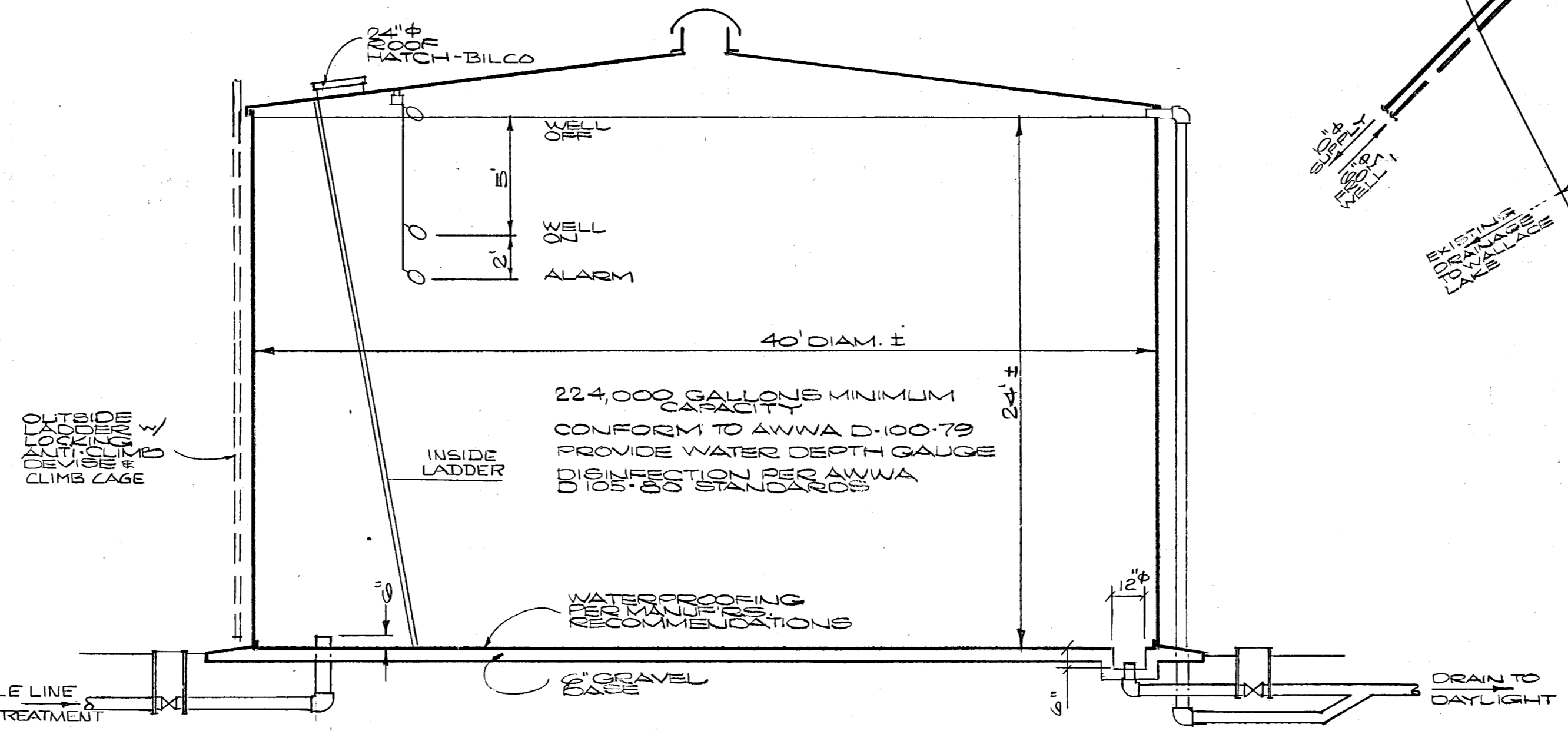
STEEL WATER STORAGE TANK SCHEMATIC SECTION
