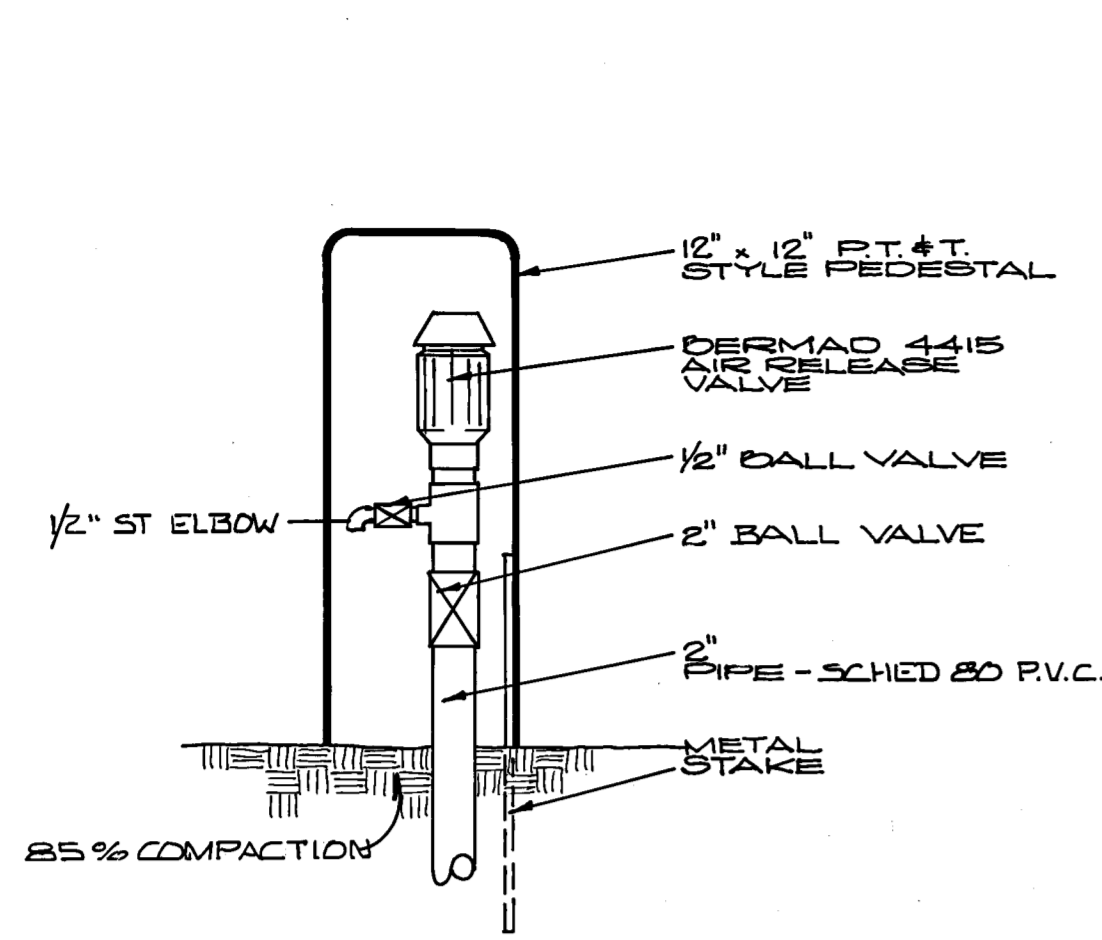
AIR RELEASE VALVE NO SCALE
