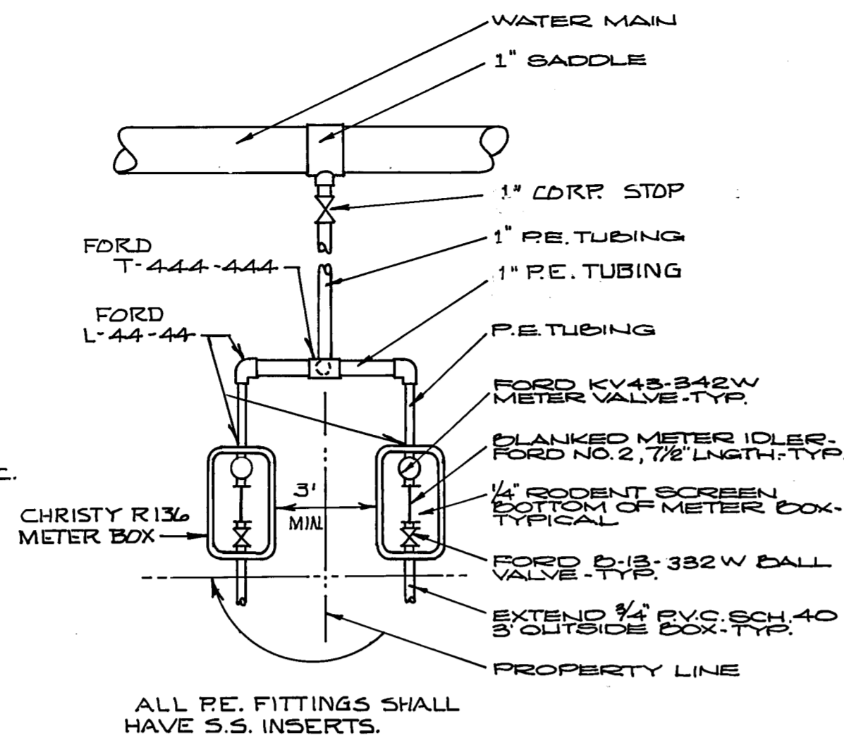
TYP. WATER SERVICE NO SCALE
