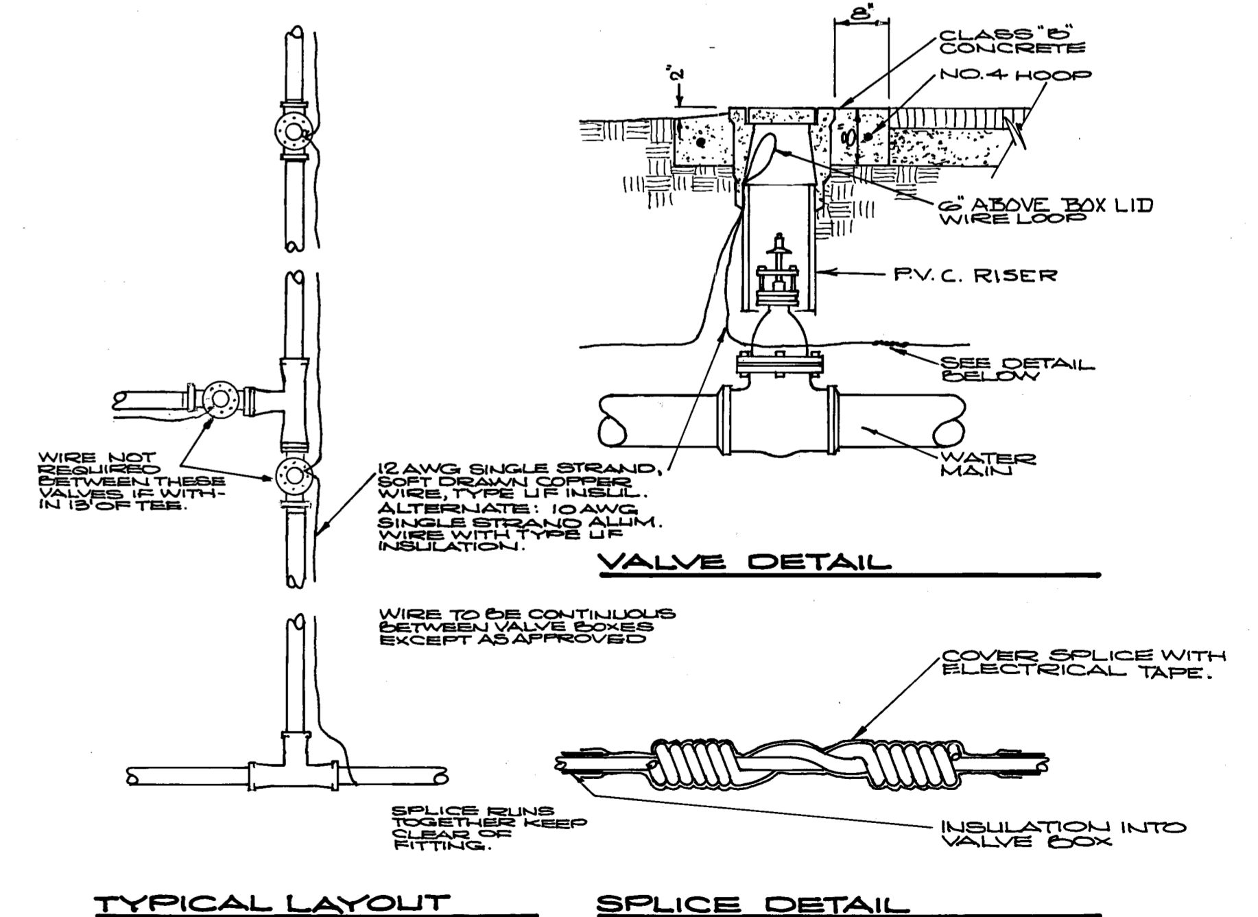
LOCATOR WIRE DETAIL NO SCALE
